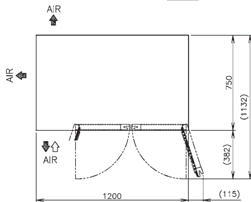
VIEW A
