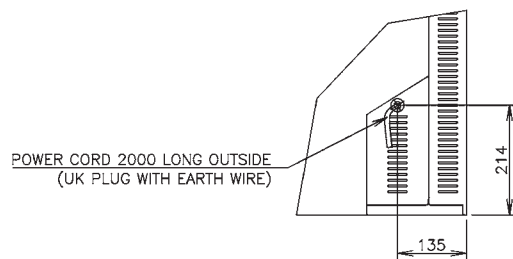
VIEW A
